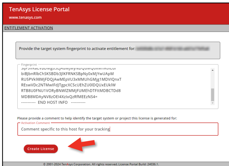
Figure 6.7 – License portal with fingerprint entered
