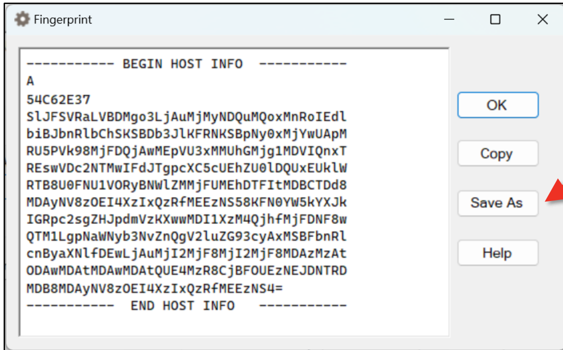
Figure 6.4 – Fingerprint
